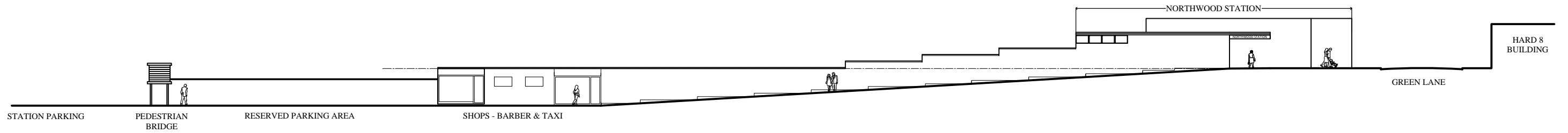
SECTION THROUGH STATION APPROACH AS EXISTING
