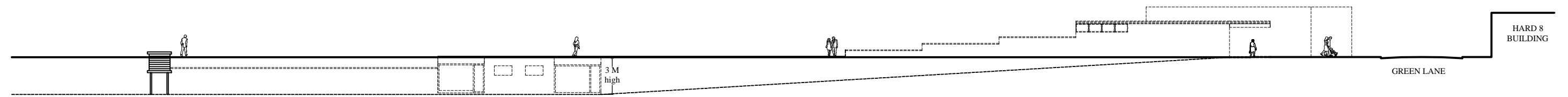
RAISED PIAZZA AS PROPOSED BY TfL - APPROX. 3 METRES ABOVE EXISTING LEVEL ON STATION APPROACH Dashed lines indicate existing levels and structures
